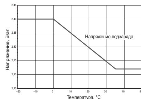
Рис. 2. Marathon M/M-FT/M-FTX/PC, Sprinter P/XP/PP, Sprinter S
